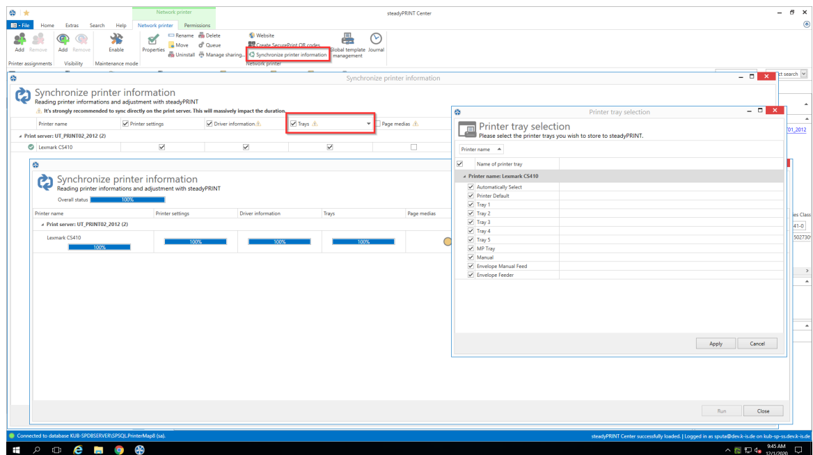
Figure 37: Overview of Input tray management
